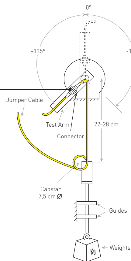
Fig 2 This paper describes the benefits of SENKO's new Mini Boots in comparison to that of standard boots in the key area of Telcordia GR-326-Core, section 4.4.3.5 T.W.A.L. compliance.
