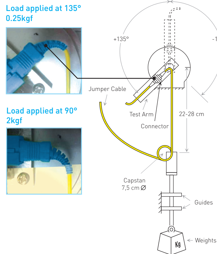
Fig 2 This paper describes the benefits of SENKO's new Mini Boots in comparison to that of standard boots in the key area of Telcordia GR-326-Core, section 4.4.3.5 T.W.A.L. compliance.
